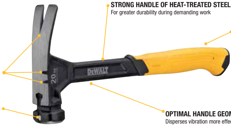
Milled hammer head
