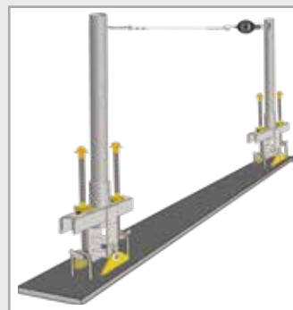
Single Span Installation
